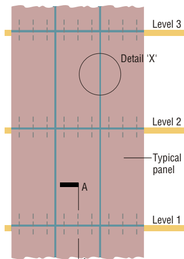
TYPICAL EXTERNAL SHEAR WALL LAYOUT
