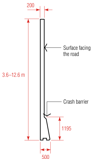
Typical sectional view of panel
