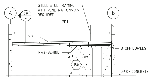
Typical section showing set-down roof panel.
