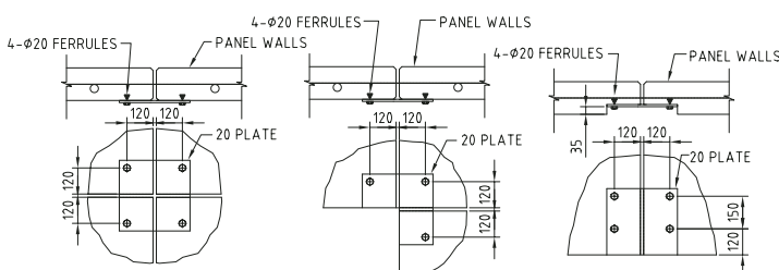
Typical wall panel connection detail.
