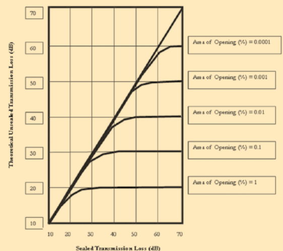
Figure 1 Insulation vs % Openings
